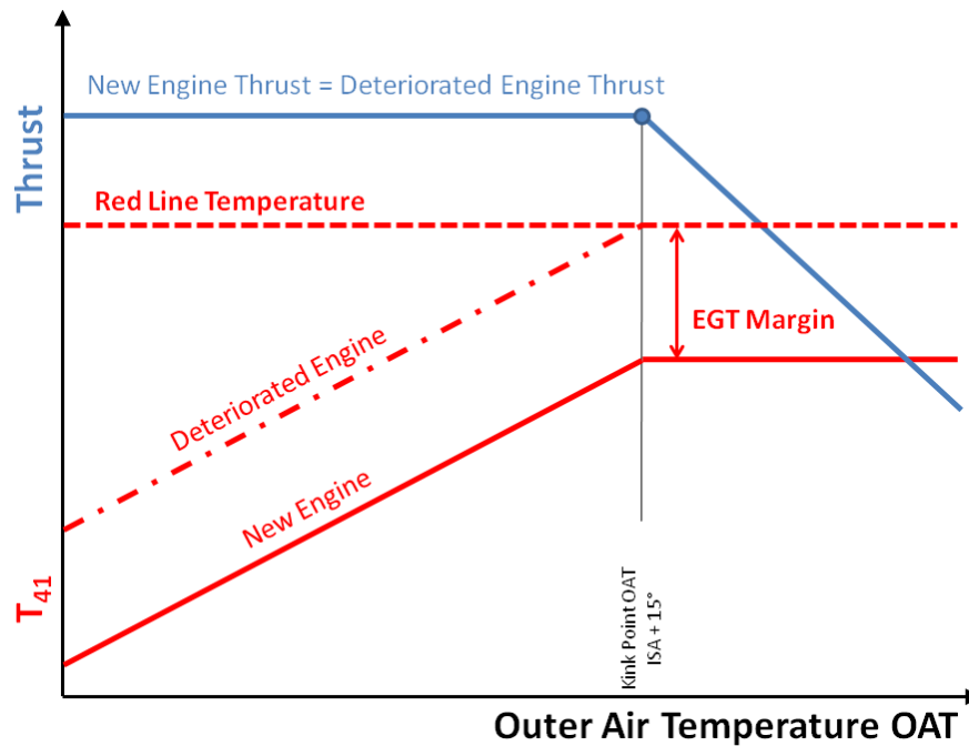
Exhaust Gas Temperature (EGT) Margin
